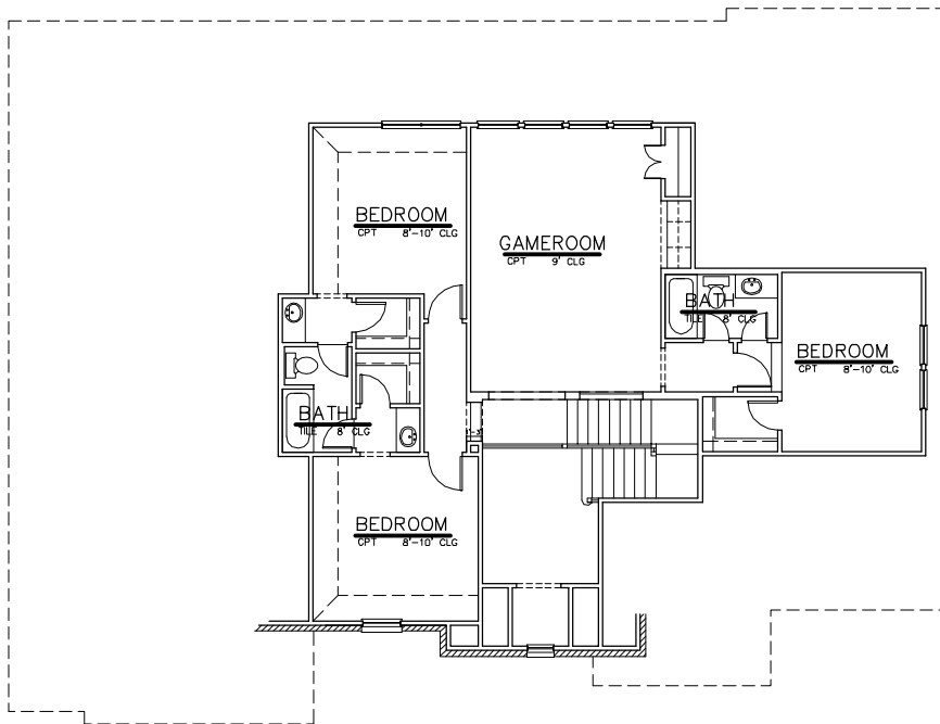
SECOND FLOORPLAN
