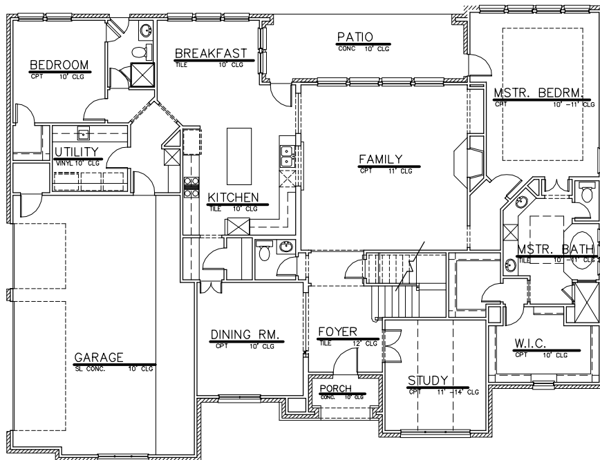
FIRST FLOORPLAN
